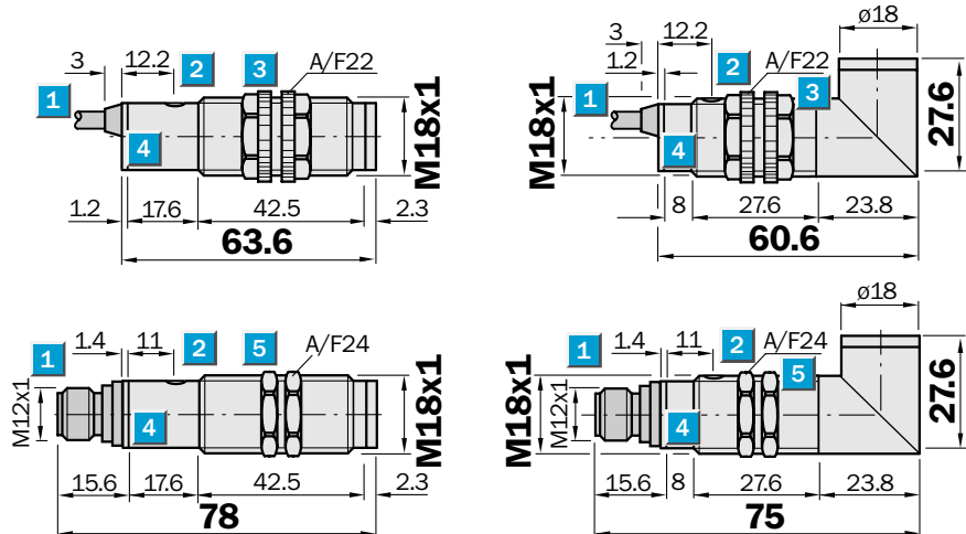
Dimensional drawing
