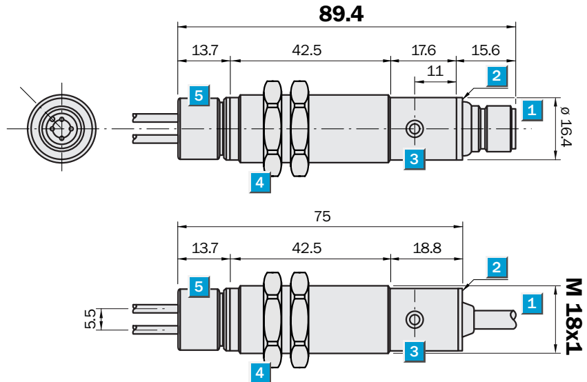
Dimensional drawing
