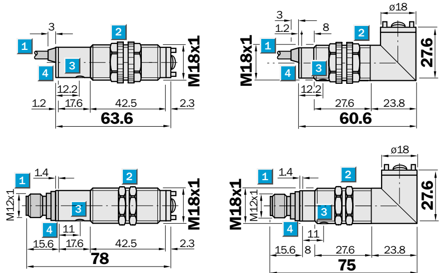
Dimensional drawing
