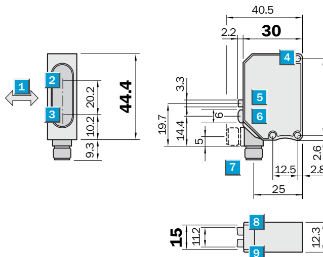
Dimension illustration
